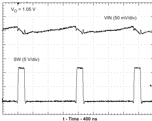
Figure 15. VOLTAGE RIPPLE AT INPUT ( I_o = 2\text{ A} )
